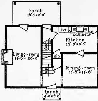
First-floor Plan
